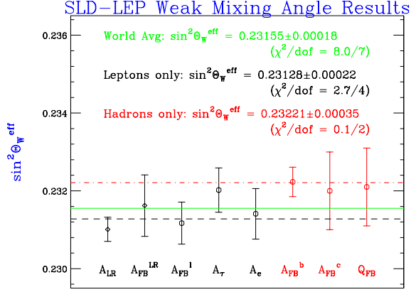
Fig. 1. Status of SLD and LEP \sin^2 \theta_W^{\text{eff}} measurement. Notice that the leptonic results are consistent with each other and different from the LEP hadronic results.
