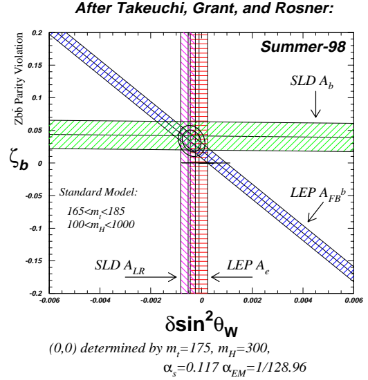
Fig. 2. Transformation of Z^0 b \bar{b} coupling parity violation versus \sin^2 \theta_W^{\text{eff}} .
