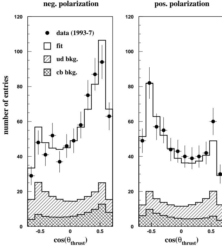
FIG. 1. Polar angle distributions of the thrust axis, signed to point in the direction of negative strangeness, of the tagged strange particle, for negative (left) and positive (right) beam polarization. The dots show data and the histogram shows our fit to the data. Our estimates of the non- s\bar{s} backgrounds are indicated by the hatched histograms.
