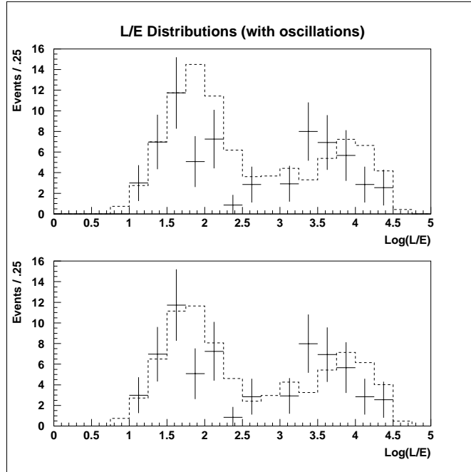
FIG. 3. L/E distribution for \nu_\mu background subtracted data with Monte Carlo expectation for \Delta m^2 = 1.0 \times 10^{-3} \text{ eV}^2 (top) and \Delta m^2 = 5.0 \times 10^{-3} \text{ eV}^2 (bottom)
