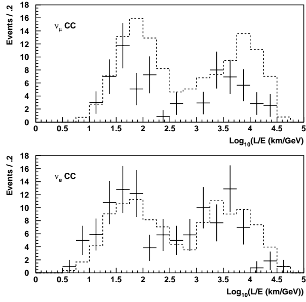
FIG. 2. L/E distributions for \nu_\mu CC and \nu_e CC background subtracted data (crosses) and the Monte Carlo expectation without oscillations (dashed histogram). The MC is normalized to 4.2 kiloton-years data.
