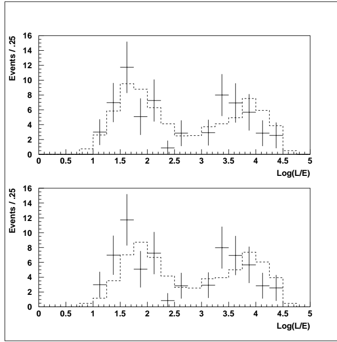
FIG. 4. L/E distribution for \nu_\mu background subtracted data with Monte Carlo expectation for \Delta m^2 = 1.1 \times 10^{-2} eV^2 (top) and \Delta m^2 = 1.0 \times 10^{-1} eV^2 (bottom). 1.1 \times 10^{-2} eV^2 is our best fit for \sin^2(2\theta) = 1.0 .
