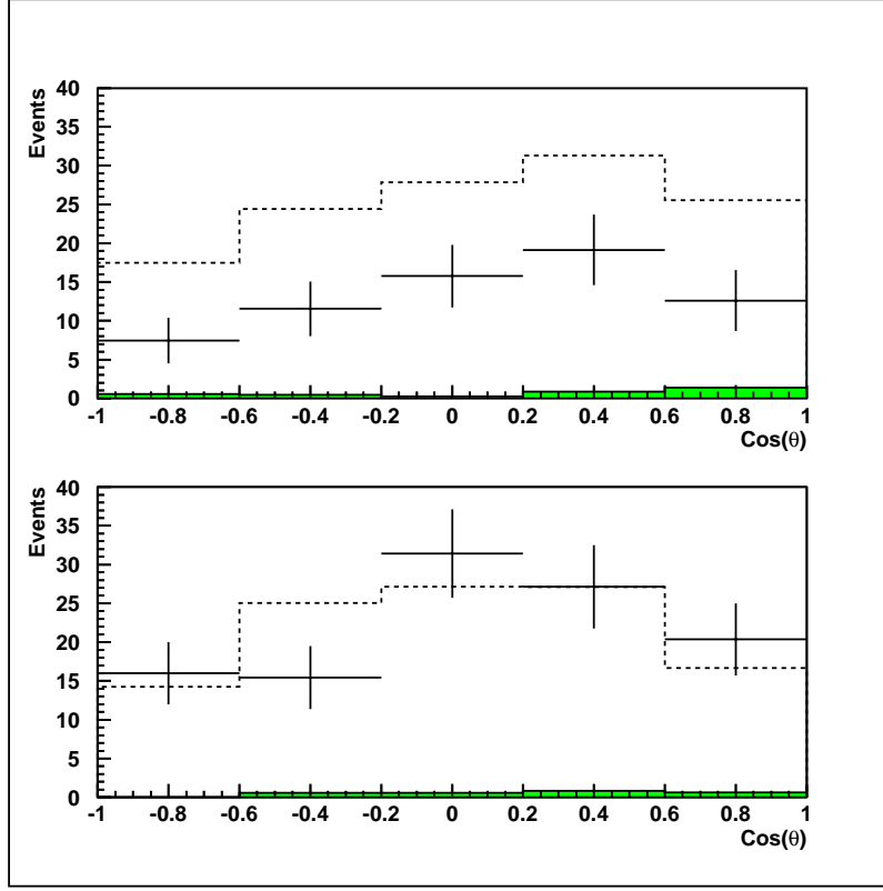
FIG. 1. The zenith angle distribution of the data (points), neutrino Monte Carlo without oscillations (dashed line) and the rock background (shaded). The upper curve is for \nu_\mu events and the lower curve for \nu_e 's. The rock and Monte Carlo curves are normalized to the data.
