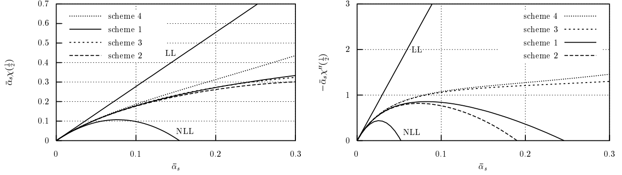
FIG. 2. The result of resumming double transverse logarithms on \chi and its second derivative, from Ref. [12].
