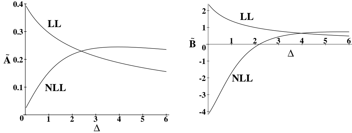
FIG. 3. Dependence of \tilde{A} = \bar{\alpha}_s \chi(\frac{1}{2}) and \tilde{B} = -\frac{1}{2} \bar{\alpha}_s \chi''(\frac{1}{2}) on \Delta for \alpha_s = 0.15 , from Ref. [3].
